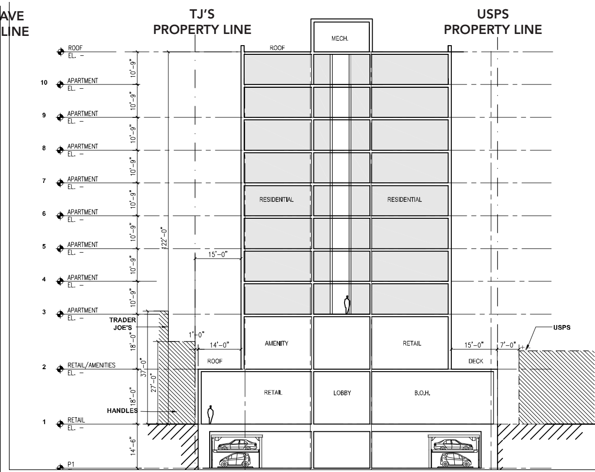
SECTION B-B
