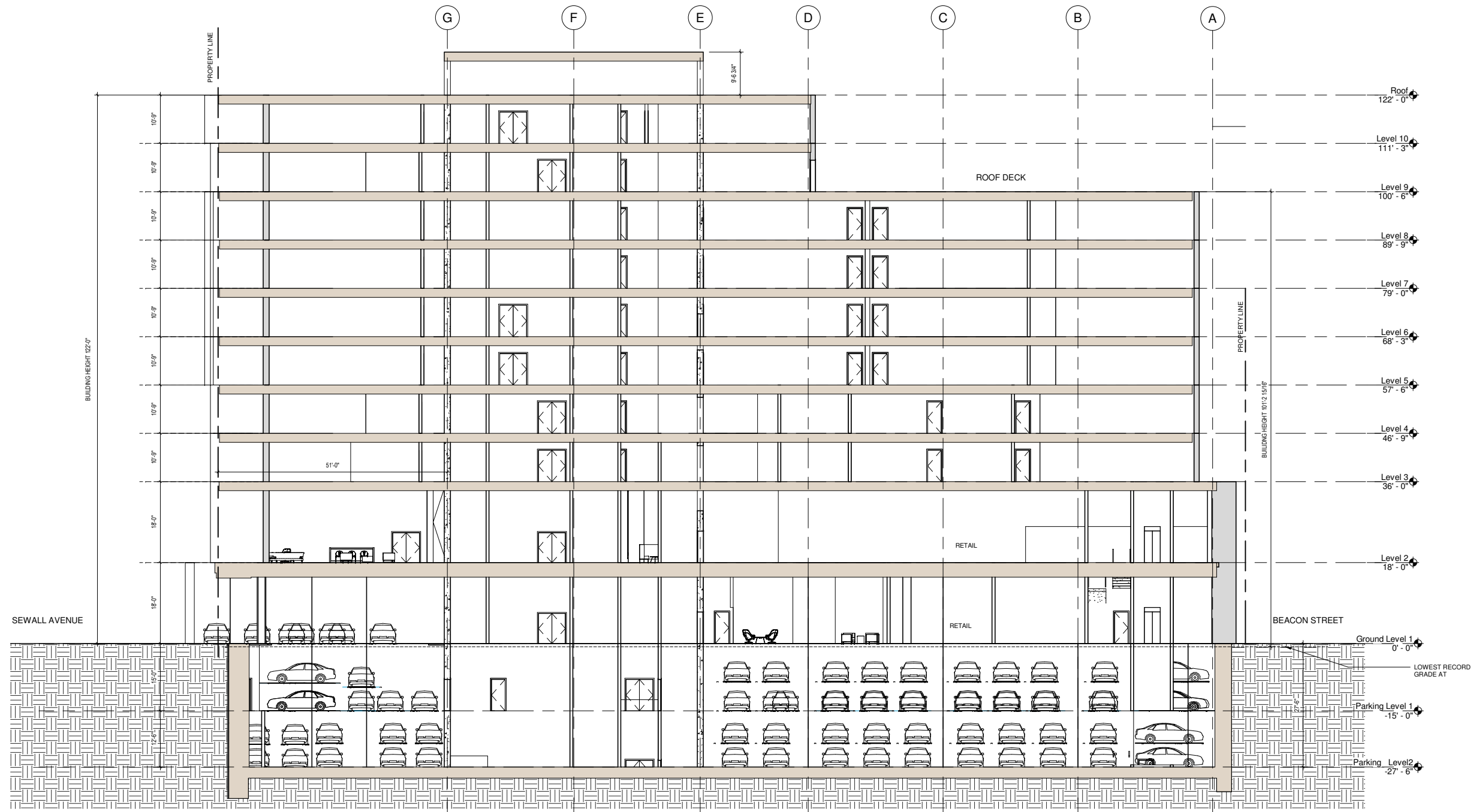
1 Max Building Height Section 3/32" = 1'-0"
