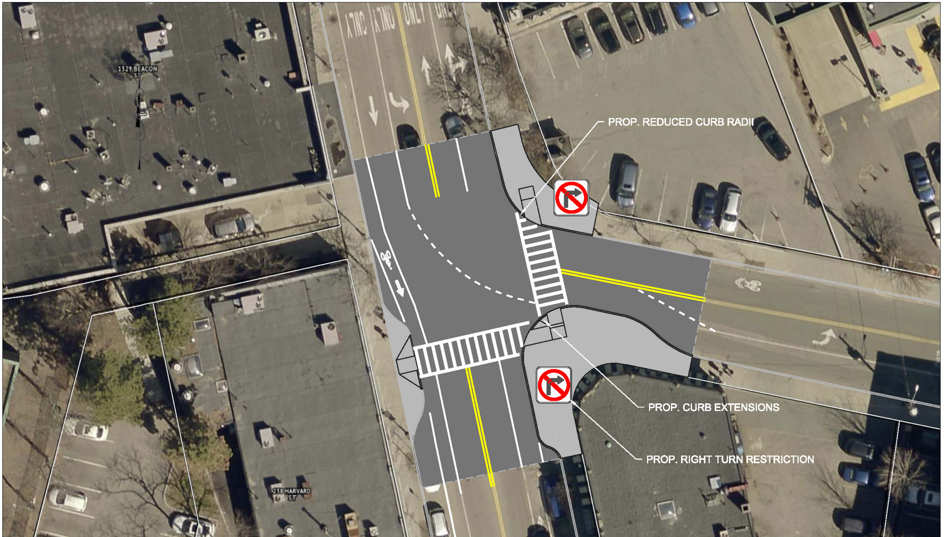
Figure 1 Longwood Avenue at Harvard Street Intersection Improvements Transportation Board Approved Plan 5-13-2019
