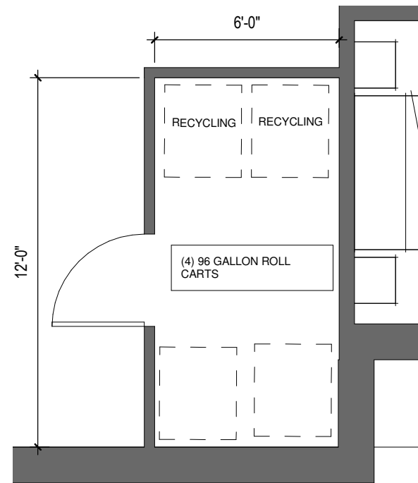
4 ENLARGED PLAN - L2 RETAIL TRASH ROOM 1/4" = 1'-0"
