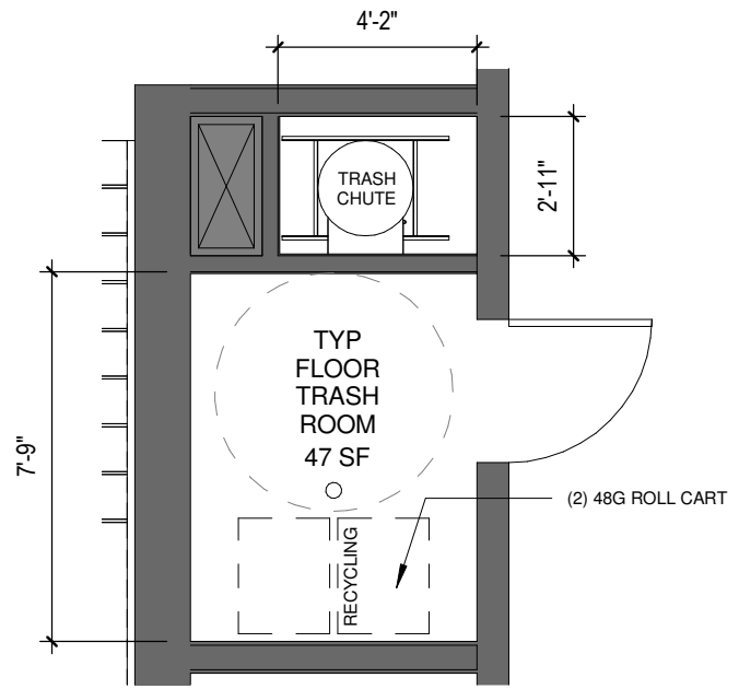
2 ENLARGED PLAN - TRASH ROOM AT TYP LEVEL 1/4" = 1'-0"
