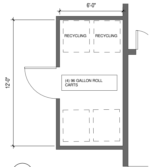
3 ENLARGED PLAN - L1 RETAIL TRASH ROOM 1/4" = 1'-0"
