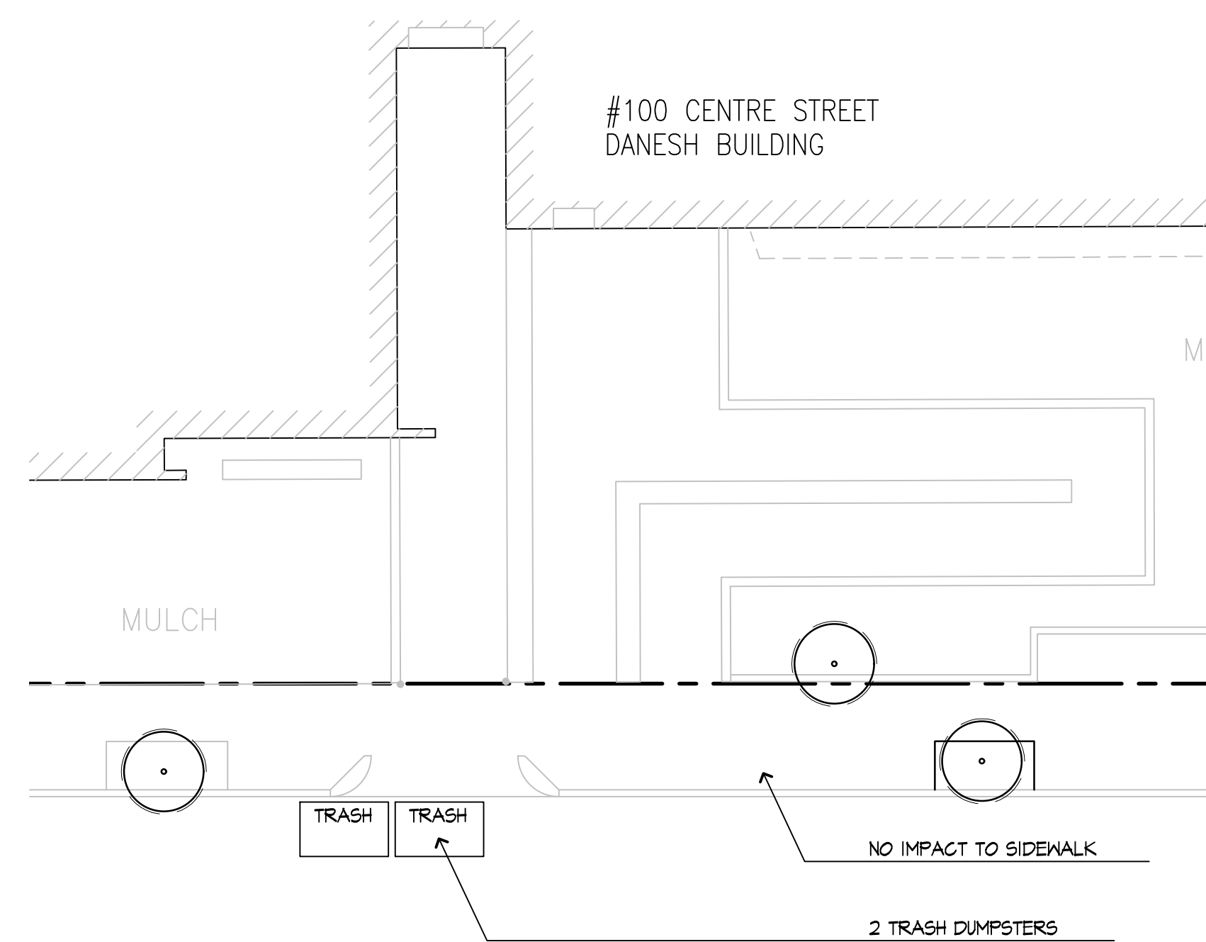
2 HSL #100 CENTRE ENLARGMENT SCALE: NTS
