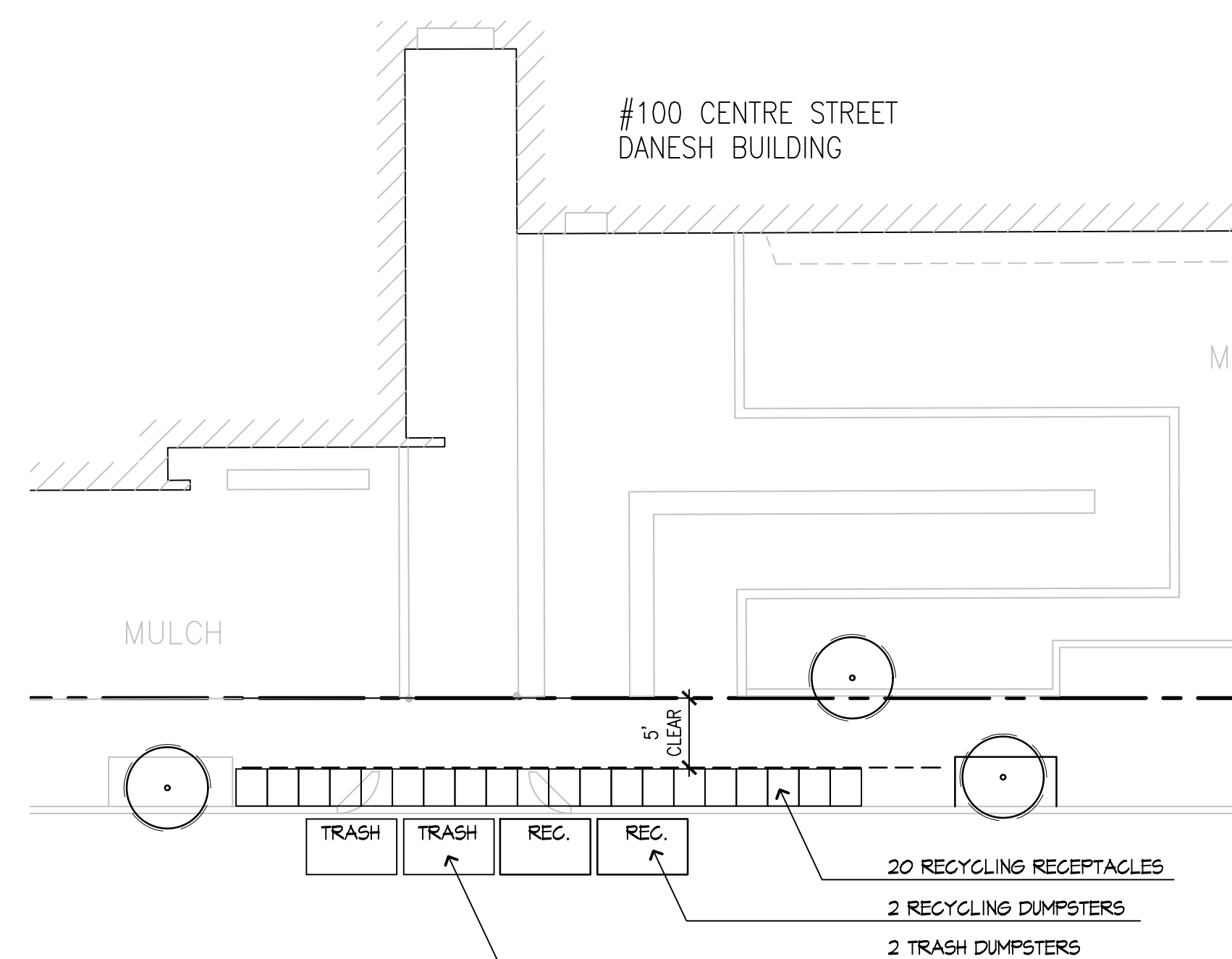
2 HSL #100 CENTRE ENLARGEMENT
